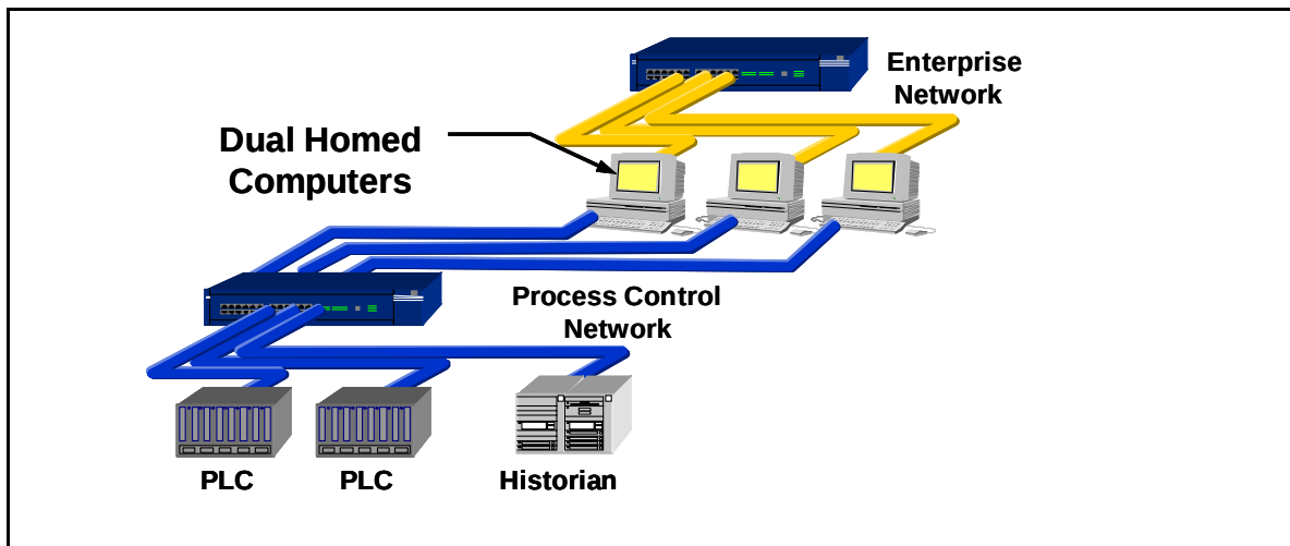
Figure 2: Network Separation Using Dual-Homed Computers
