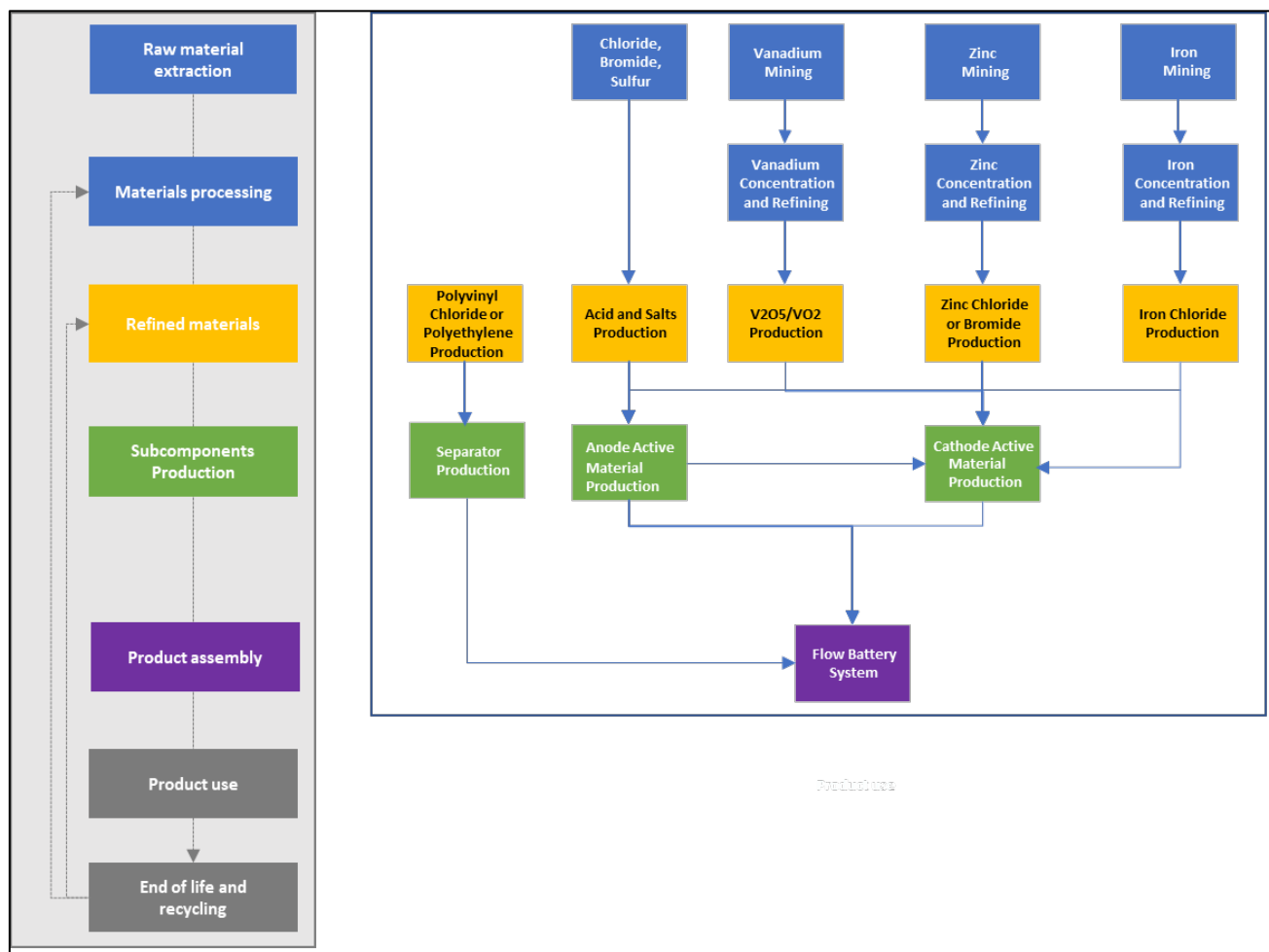
Figure 18. Flow battery supply chain.
