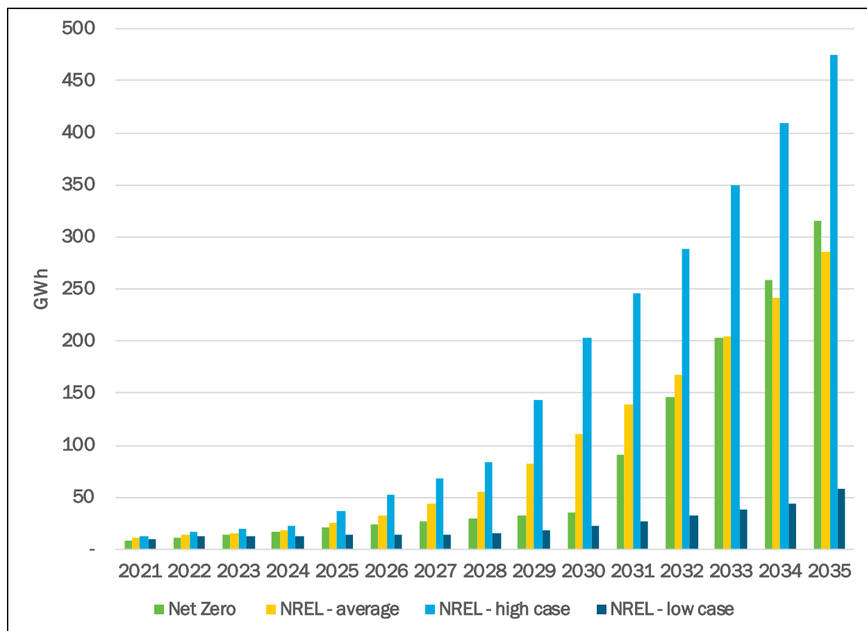
Figure 9. Scenario projections of cumulative U.S. grid storage capacity.
