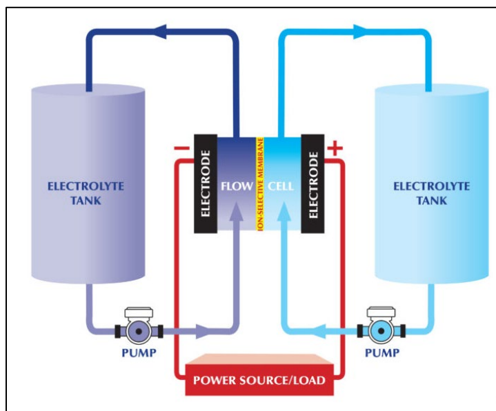
Figure 2. Flow battery schematic.
