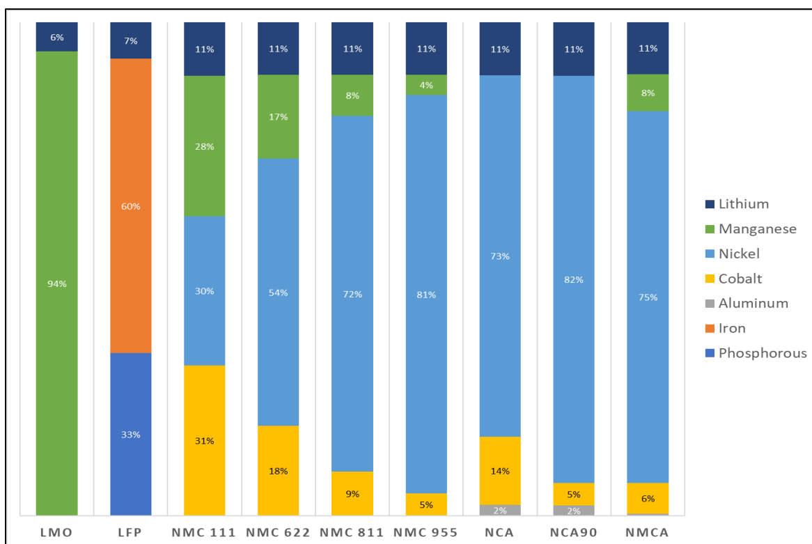
Figure 1. Metal content (wt%) of lithium-ion battery cathodes.
