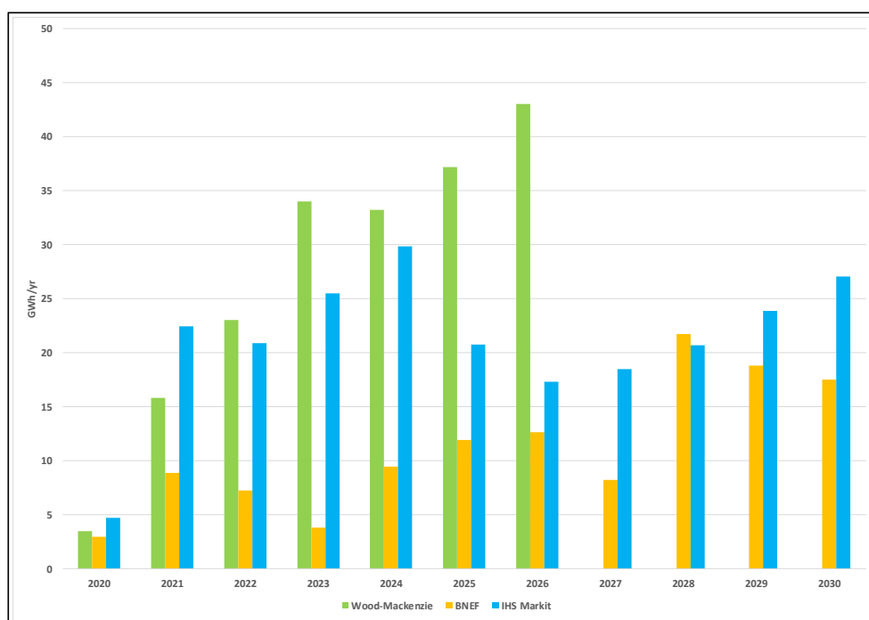
Figure 4. Projected U.S. annual grid storage.
