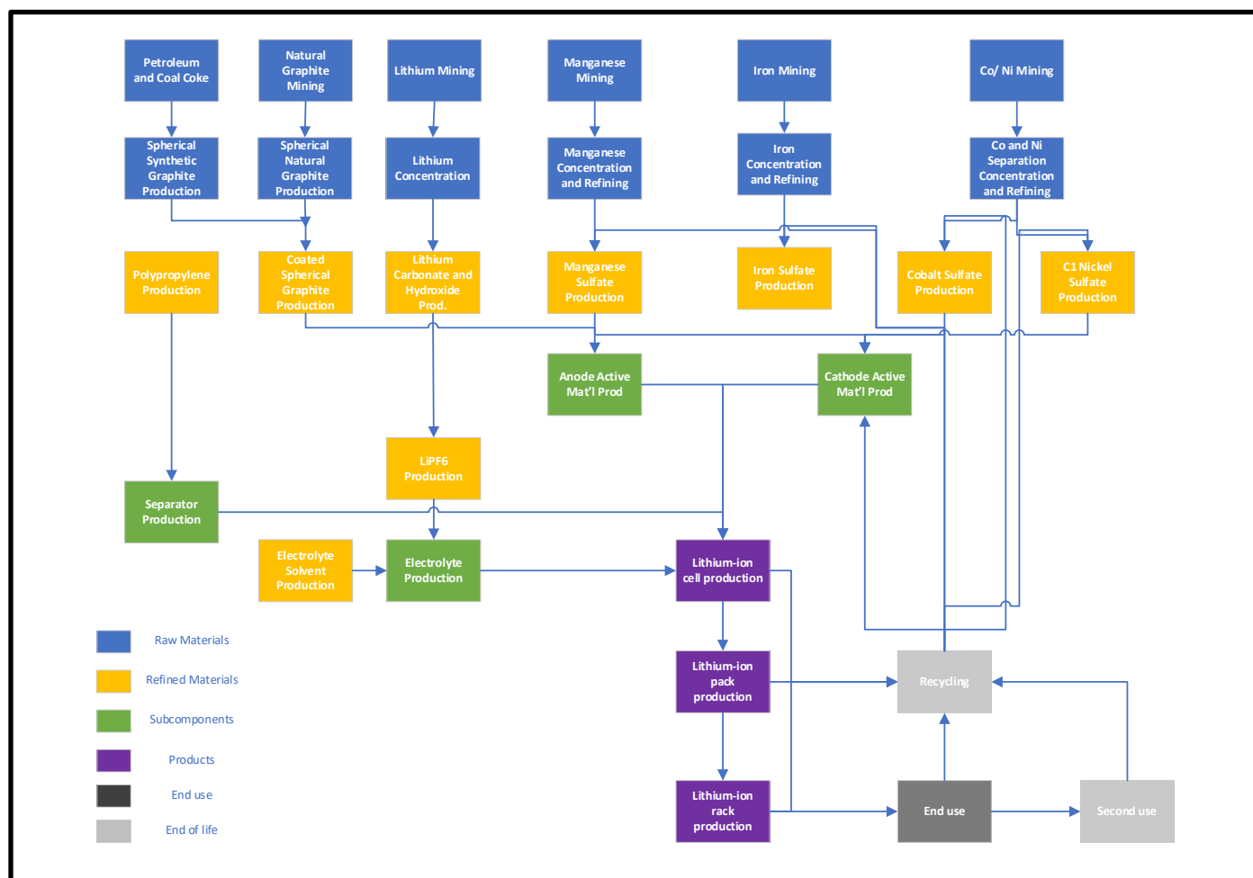
Figure 11. Lithium-ion Battery Supply Chain Diagram
