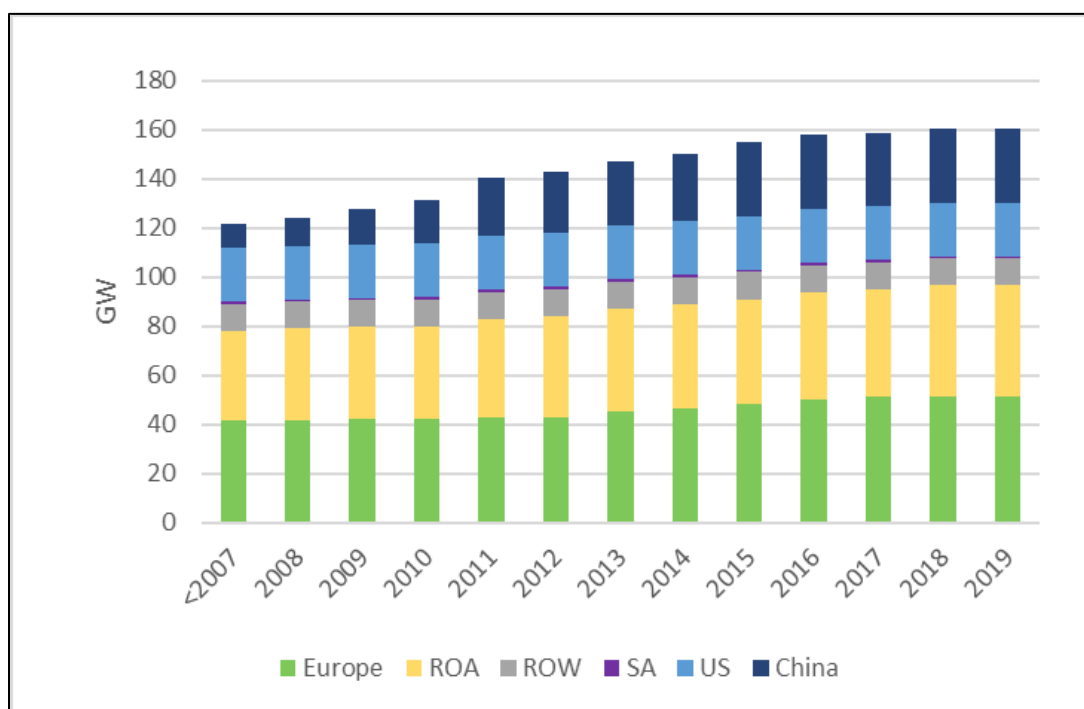
Figure 5. Global cumulative PSH deployment. 8
