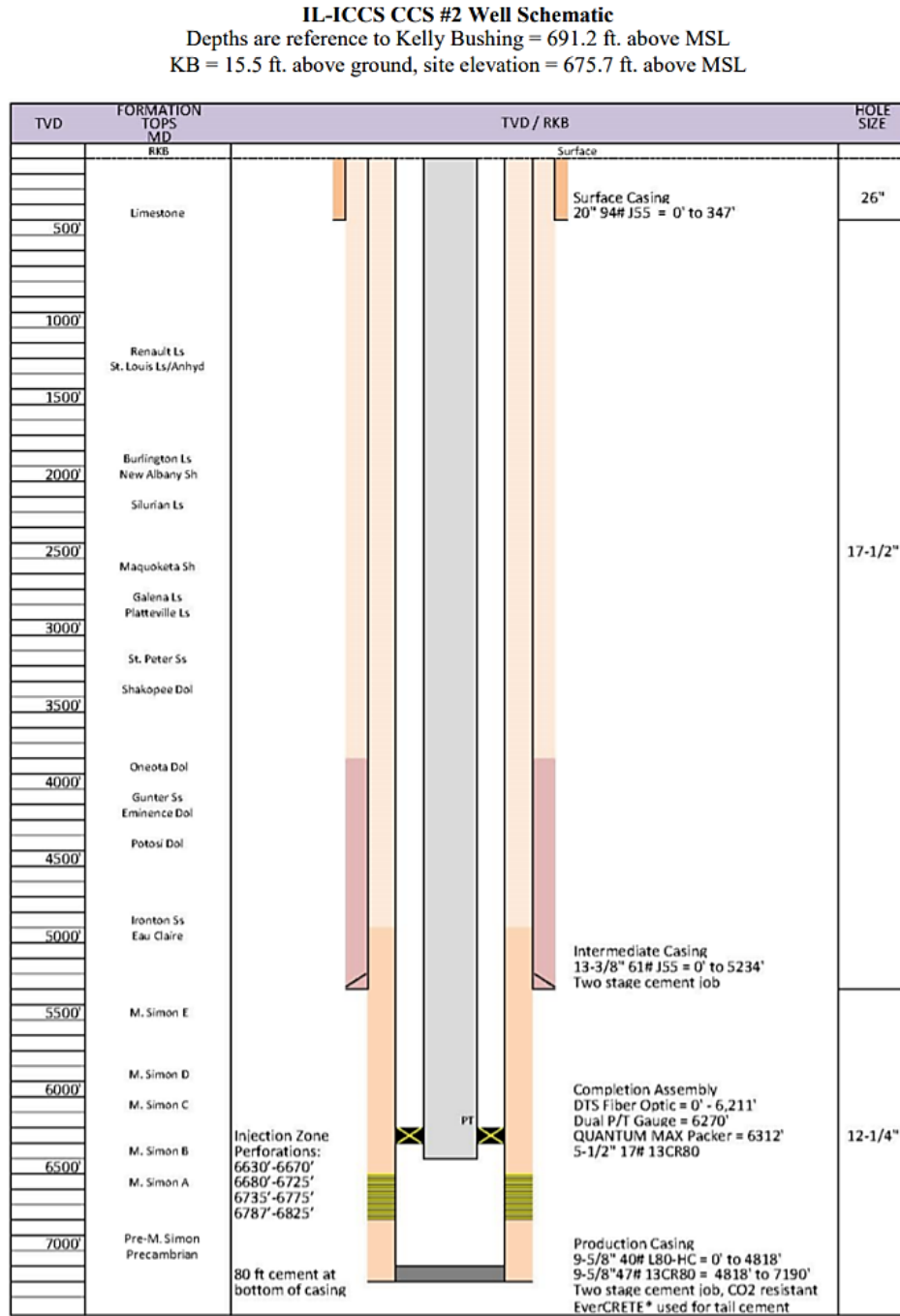
Figure 22: Archer Daniels Midland CCS#2 well schematic representing typical casing and cement program for CO 2 injector well 46
