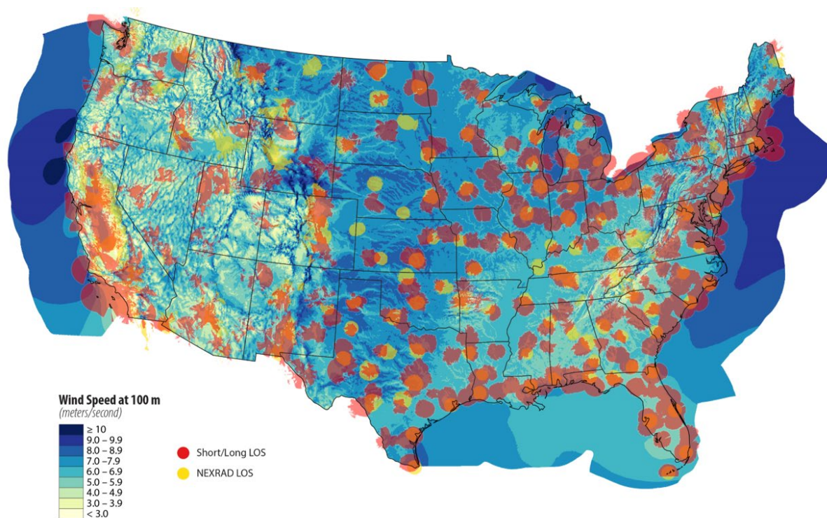
Figure 1 – This map shows radar line-of-sight (LOS) polygons approximated at 100 meters above ground using a simple viewshed analysis based on publicly available radar station locations. The polygons do not represent the actual line-of-sight that can be observed by the scan of a radar system but give an approximation of the potential areas of CONUS where wind turbine build out may impact a radar system. Short/Long (red shading) range refers to air traffic control and air route surveillance radars respectively and NEXRAD (yellow shading) represents weather radars. The yellow and red shading is for visualization purposes only and these areas do not represent no-go zones for wind development. Image created by the National Renewable Energy Laboratory.
