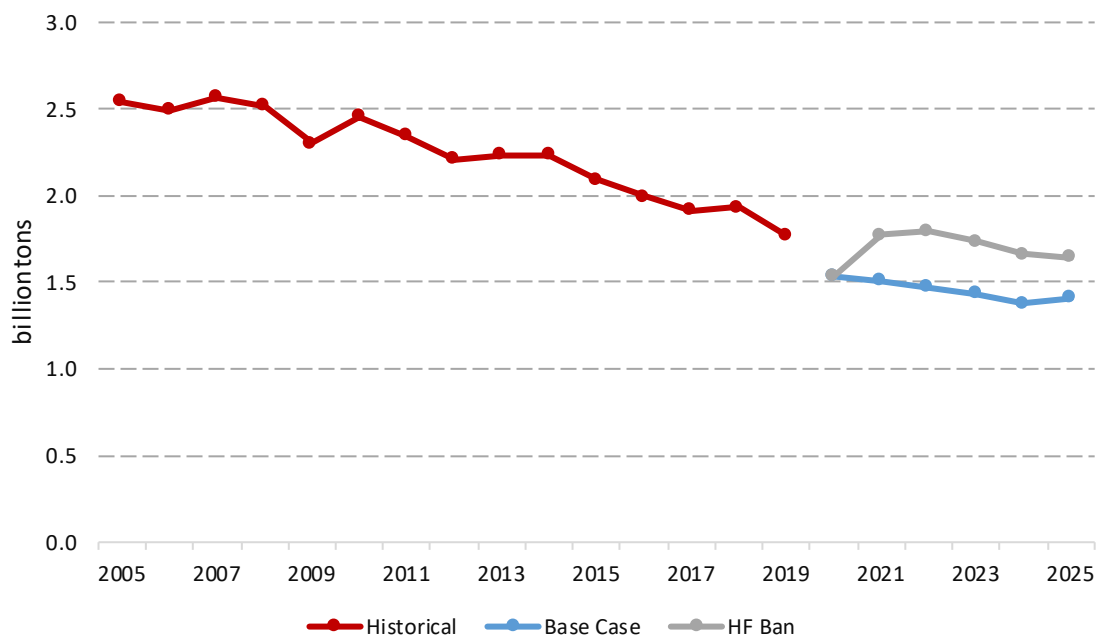
Figure 39: Historical and Projected CO 2 Emissions (2005-2025)
